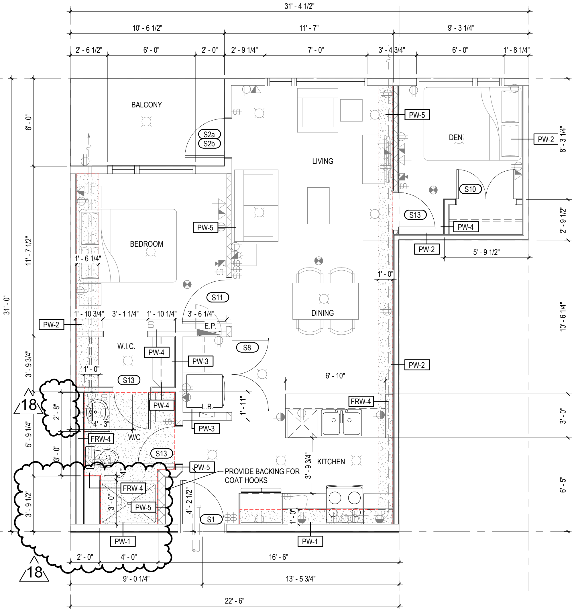
1 B SUITE - 732ft 2 A220 1/4" = 1'-0"
