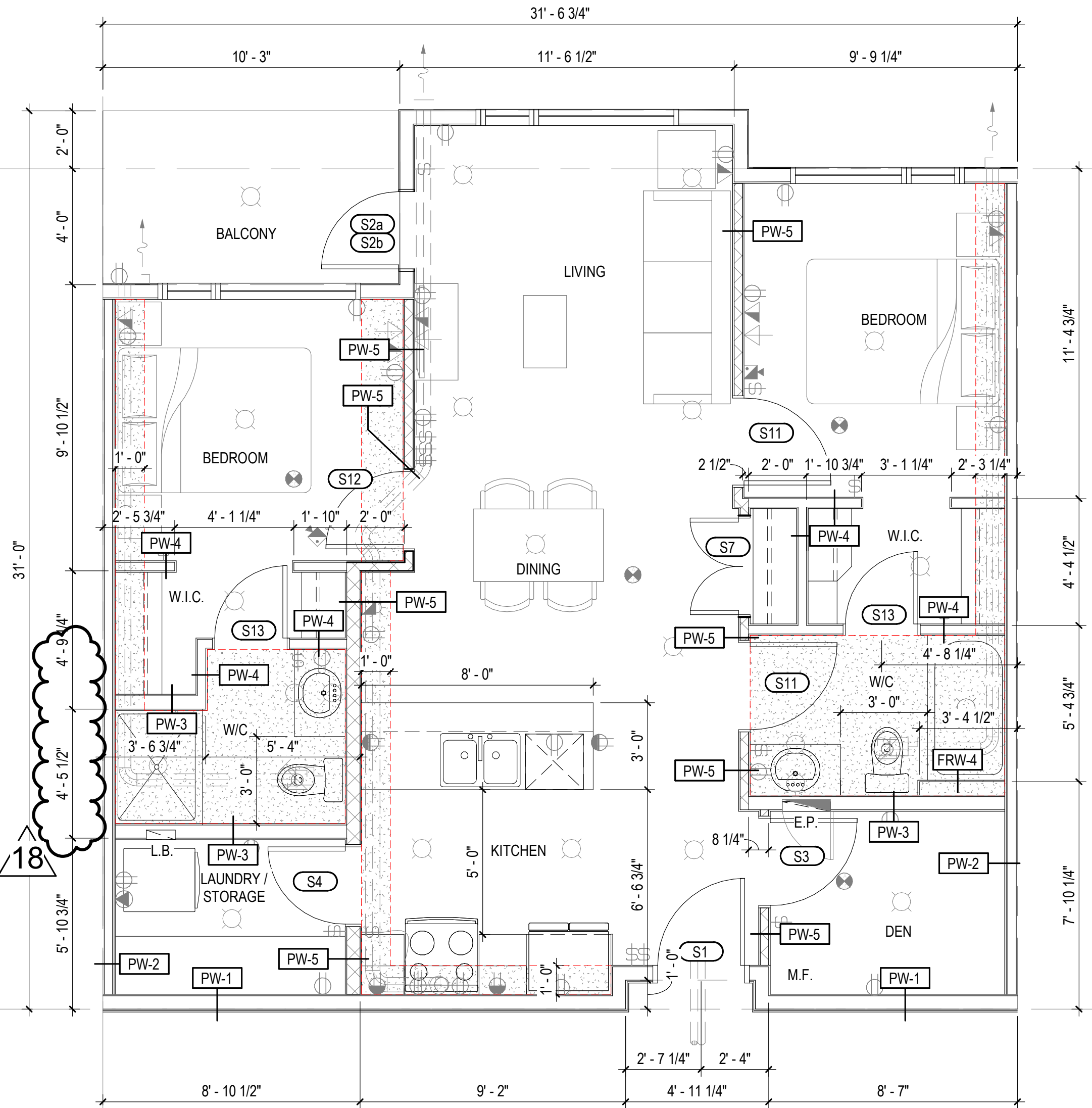
4 B3 SUITE - 894ft 2 A220 1/4" = 1'-0"
