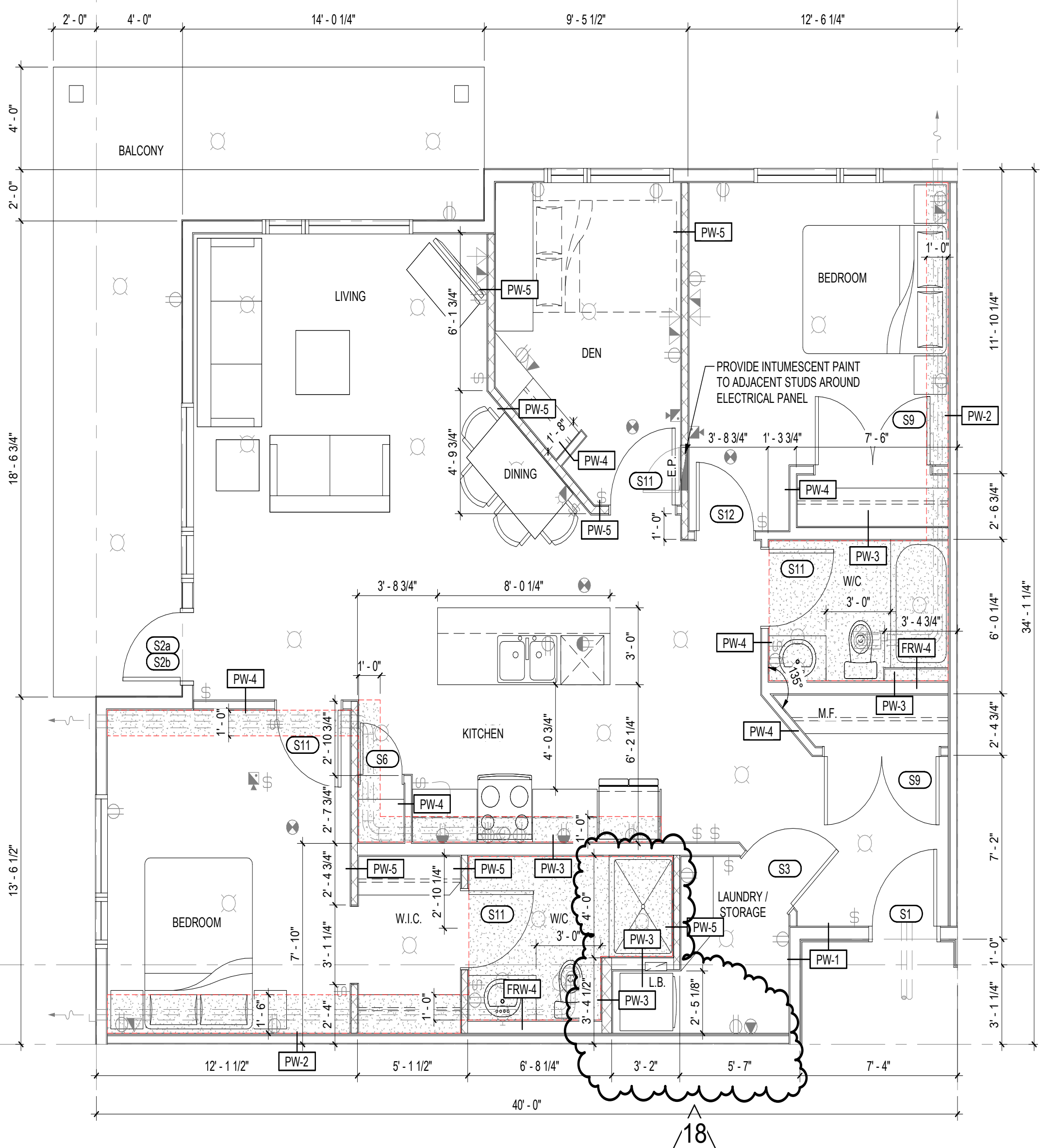
6 C SUITE - 1224ft 2 A220 1/4" = 1'-0"
